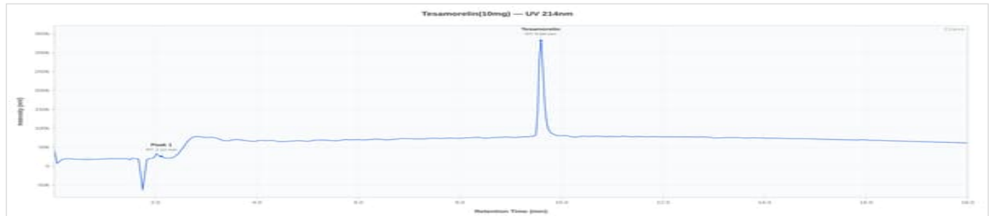
Tesamorelin 10mg - TES-10MG-0924A: UV Chromatogram
